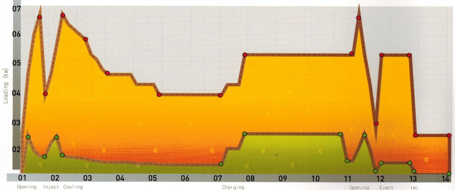
POWER CONSUMPTION CURVE BETWEEN TRADITIONAL HYDRAULIC AND HYBRID SYSTEM
